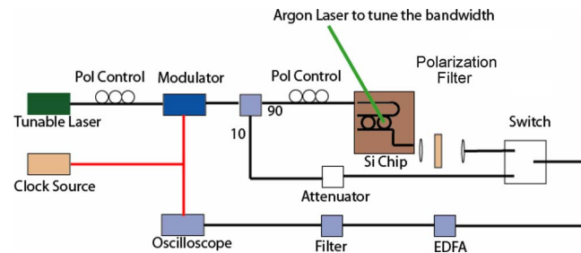
Fig. 4. (Color online) Experimental setup. The black lines represent optical fiber. Lines connecting modulator rf input and oscilloscope trigger input represent coaxial cables. A high speed electro-optic modulator generates a sinusoidal probe beam of 500 MHz. Light is coupled to the device and compared with a reference arm to determine the delay or advance. An argon laser beam at 514.5 nm is used to thermally tune the structure to vary the bandwidth of the induced absorption feature.
