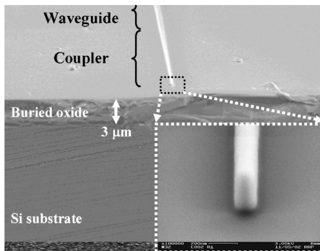
Fig. 3. Scanning electron microscopy pictures of a typical nanotaper coupler, showing an enlarged view of the tip.
