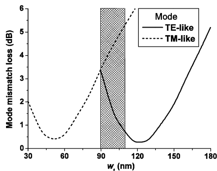
Fig. 2. Mode mismatch loss dependence on nanotaper tip width. The crosshatched region represents the range of experimental values of w_t .
