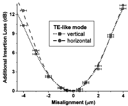
Fig. 4. Additional insertion loss of the nanotaper caused by fiber-coupler transverse misalignment for a TE-like mode at \lambda_0 = 1550 nm.
