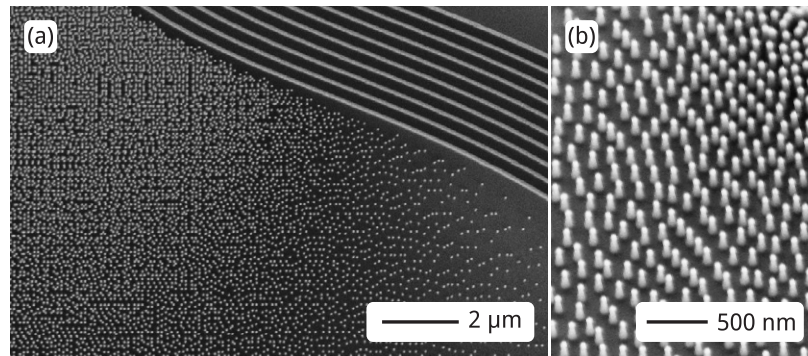
Figure 4. Fabrication of the TO devices. (a) Dithered pattern on silicon showing the different densities of silicon pillars from higher (upper left) to lower (bottom right). The lines on the upper right are a distributed Bragg reflector that was part of this device. (b) Zoomed view of the silicon pillars on an intermediate density region.
