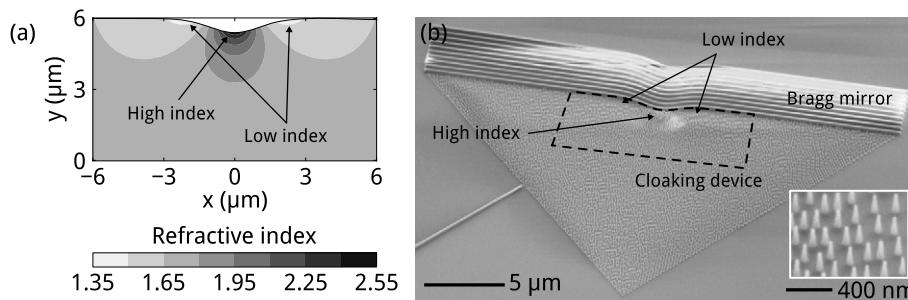
Figure 5. Cloaking device. (a) Initial refractive index map of the cloaking device. (b) SEM image of the fabricated device. The map (a) corresponds to the main cloaking device (dashed area). The inset is a zoomed-in view of the Si nano-structures that compose the device.
