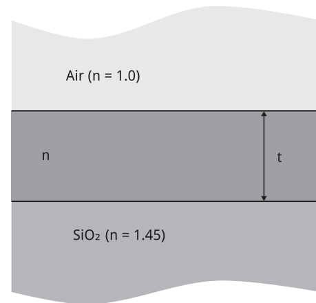
Figure 2. Schematic of an air-cladded slab waveguide on SiO 2 substrate.
