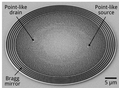
Figure 7. SEM of the fabricated Maxwell's fish eye with a distributed Bragg reflector surrounding it. The source and drain (where the image is formed) are based on gold dots used to scatter light into and out of the device layer.
