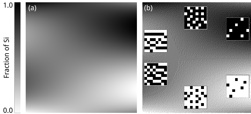
Figure 3. Example of grey-scale map dithering. (a) The grey-scale map [\rho]_{M,N} indicates the volumetric fraction of Si at every point of the device slab. (b) The dithering process quantizes the map into nanometre size regions composed either of Si or air, preserving the overall shades of grey. The insets show regions with 10\times magnification.
