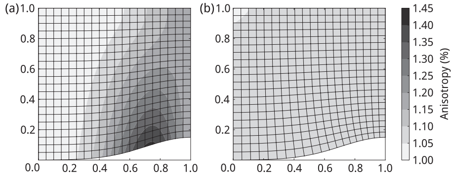
Figure 1. Example of anisotropy minimization (measured as the ratio between the maximal to the minimal refractive indices along the two principal axes of the medium [7]). Here we transform a square space in the one defined by the boundaries in the figures. The grid lines show how a square grid in the original space is transformed inside the boundaries. (a) Initial transformation guess based on a linear interpolation of the boundaries. Anisotropy reaches 1.41. (b) Without changing the boundaries, the transformation is optimized to minimize the anisotropy of the medium to a maximum of 1.09.
