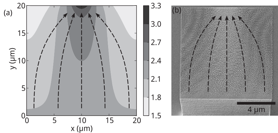
Figure 6. Light concentrator. (a) Refractive index map of the device. Light from the bottom is concentrated towards a tighter spot on the centre of the top edge where the refractive index is higher. (b) SEM image of the fabricated device corresponding to the dithered version of the designed index gradient. The arrows indicate how light travels in the device and concentrates towards the top edge.
