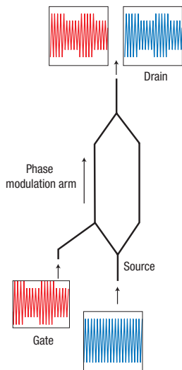
Figure 1 The all-optical modulator that breaks speed limits 5 . The gate signal (red) has its intensity modulation transferred to the source signal (blue) through nonlinear phase modulation in one arm of the interferometer. The whole structure consists of a silicon waveguide clad with a specially engineered nonlinear polymer and could be manufactured using conventional back-end silicon technology. With operation frequencies larger than 1 THz, the modulator is two orders of magnitude faster than existing silicon devices.
