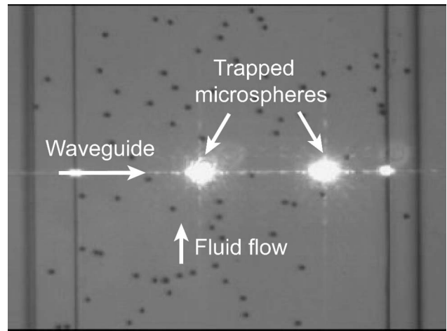
Fig. 3. Optical trapping and transport of 3- \mu\text{m} -diameter polystyrene microspheres in a microfluidic channel using a supercontinuum broadband light source. Video (Media 1) (medioref) shows optical trapping of several polystyrene microspheres using \sim 10 mW of guided power. Playback is 2 \times real time.
