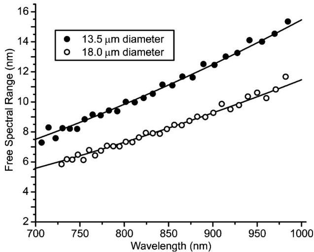
Fig. 5. Experimental (circles) free spectral range in microspheres of different diameters with theoretical (solid lines) curves for WGMs in spherical cavities.
