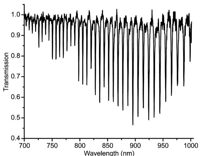
Fig. 4. Waveguide transmission spectrum showing WGM resonances of an optically trapped 18- \mu\text{m} -diameter polystyrene microsphere with quality factors of \sim 2,000 .
