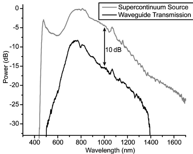
Fig. 2. Spectra of the supercontinuum source and waveguide transmission showing efficient broadband coupling to the waveguide from 700 nm to 1400 nm.
