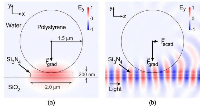
Fig. 1. (Color online) 3D simulation results for the electric field ( E_y ) profile of the quasi-TM mode at a wavelength of 850 nm in a silicon nitride waveguide. The optical forces on a dielectric microsphere can be decomposed into a transverse gradient force ( F_{\text{grad}} ) that traps the sphere to the waveguide surface and a longitudinal force ( F_{\text{scatt}} ) that propels it along the direction ( z axis) of light propagation.
