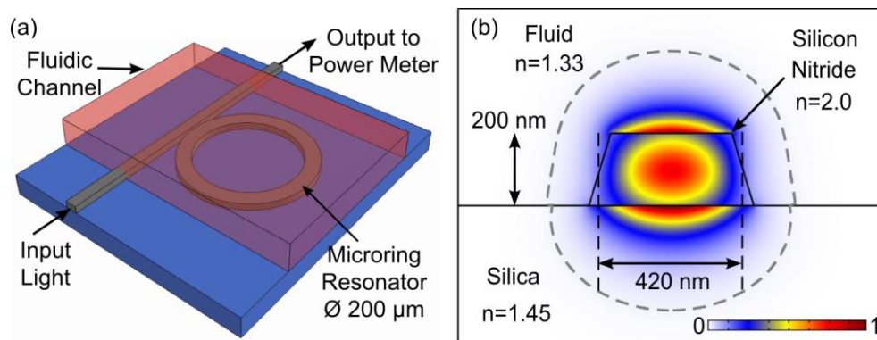
Fig. 1. (a) Device design for a microring resonator covered by a microfluidic channel. The microring enhances the interaction length between the cladding fluid and the evanescent field of the guided mode. (b). Numerical simulation of the |E|^2 profile of the TM mode in a silicon nitride waveguide at a wavelength of 650 nm and covered with an aqueous solution. The dashed line is the contour at which the field decays to 1% its maximum value.
