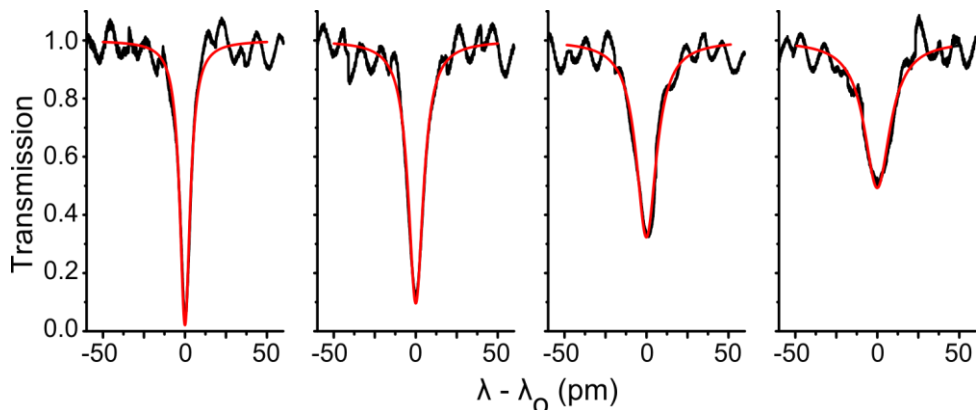
Fig. 2. Experimentally measured transmission spectrum of a microring resonator (black line) with fluid analytes of increasing absorbance (left to right) showing the change in extinction ratio and linewidth as the resonator loss increases. The data was fit (red line) using Eq. (1) to extract the absorption coefficient of the cladding fluids.
