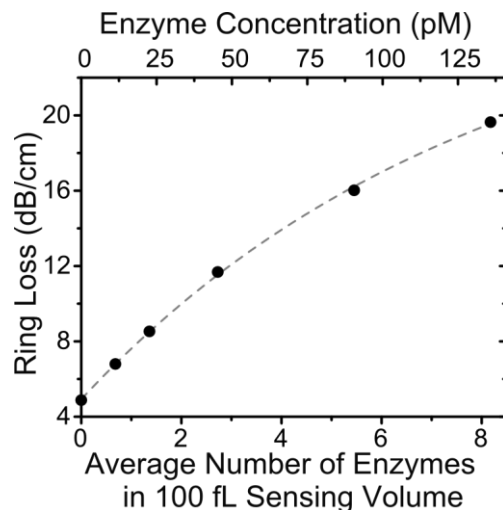
Fig. 4. Ring propagation loss as a function of both enzyme concentration and the number of enzymes within the sensing volume of the microring resonator (~100 fL).
