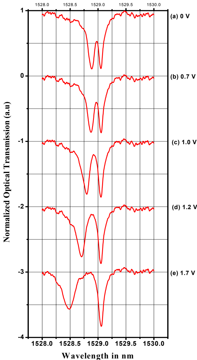
Fig. 3: Measured Optical Transmission Spectra. (a)-(e) correspond to different applied voltages. Successive curves are offset by 1 for clarity. (a) 0 V, 0 A b) 0.7 V, 4 \mu A c) 1.0 V, 100 \mu A d) 1.2, 237 \mu A e) 1.7 V, 637 \mu A applied to the ring corresponding to the left resonance.
