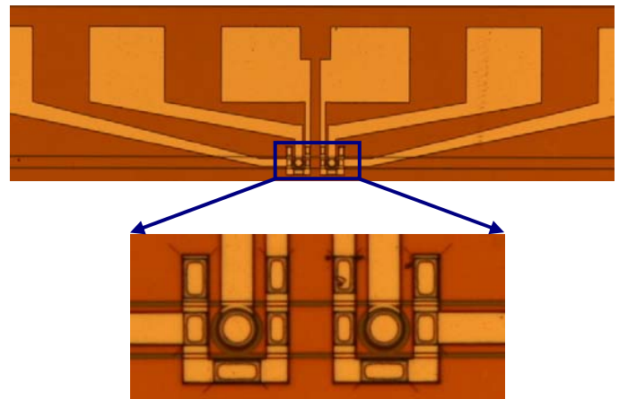
Fig. 2: Top view microscope picture of double ring resonators embedded in PIN diodes
