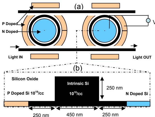
Fig. 1: a) top view schematic double ring resonators embedded in PIN diodes b) Cross section of a waveguide embedded into a PIN diode
